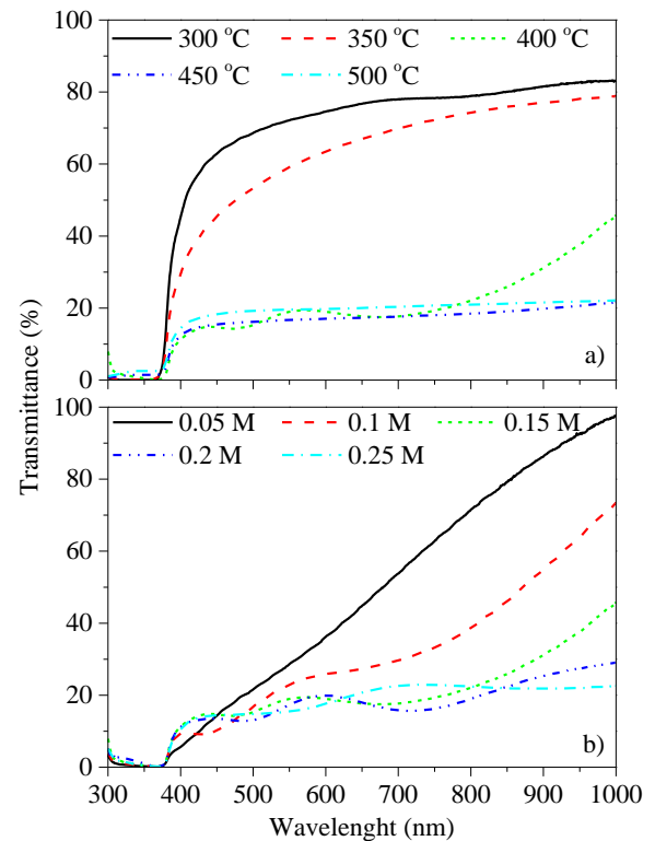
Figure 6. Optical transmittance spectra of the ZnO thin films for a) different substrate temperatures and b) different molarities.
